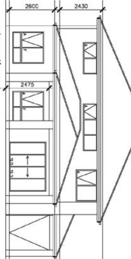
elevation A scale 1:100
